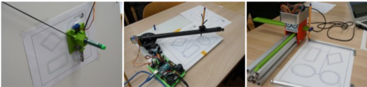
Fig 2. Different solutions to the drawing robot task. Left: Using timing belts and pulleys to draw on a vertical board. Middle: Using a combination of rotatory and linear movement to draw in polar coordinates. Right: Using two linear gears to draw horizontally.
